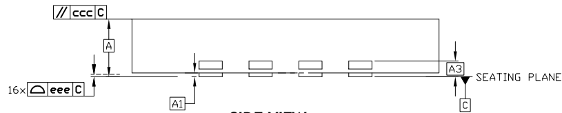
SIDE VIEW
