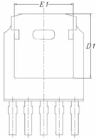
BOTTOM VIEW
