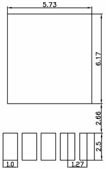
TYPICAL RECOMMENDED LAND PATTERN
