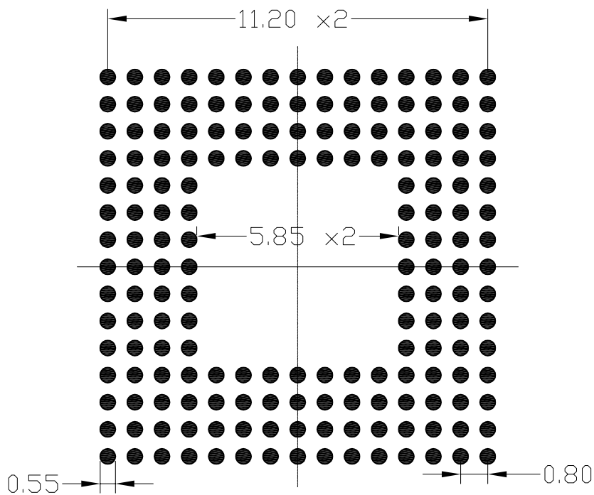
TYPICAL RECOMMENDED LAND PATTERN
