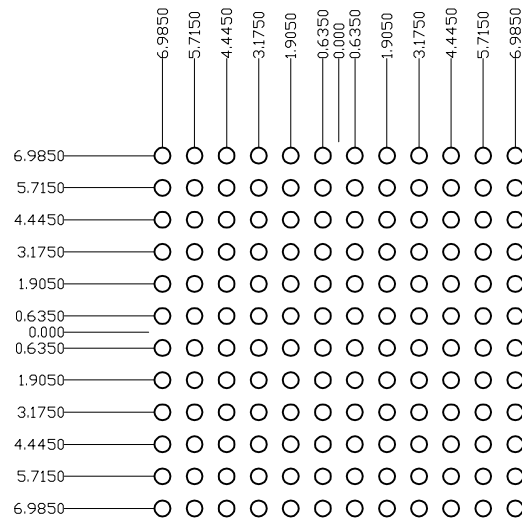
PAD LOCATION
