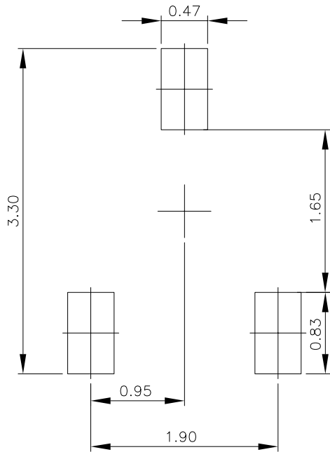
TYPICAL RECOMMENDED STENCIL
