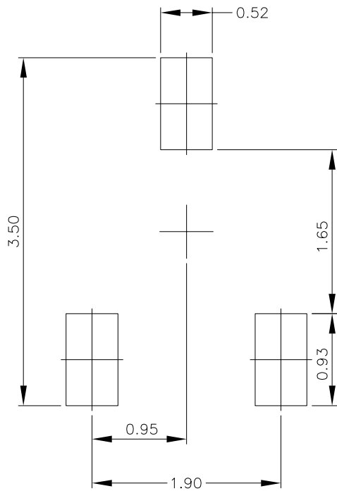
TYPICAL RECOMMENDED LAND PATTERN
