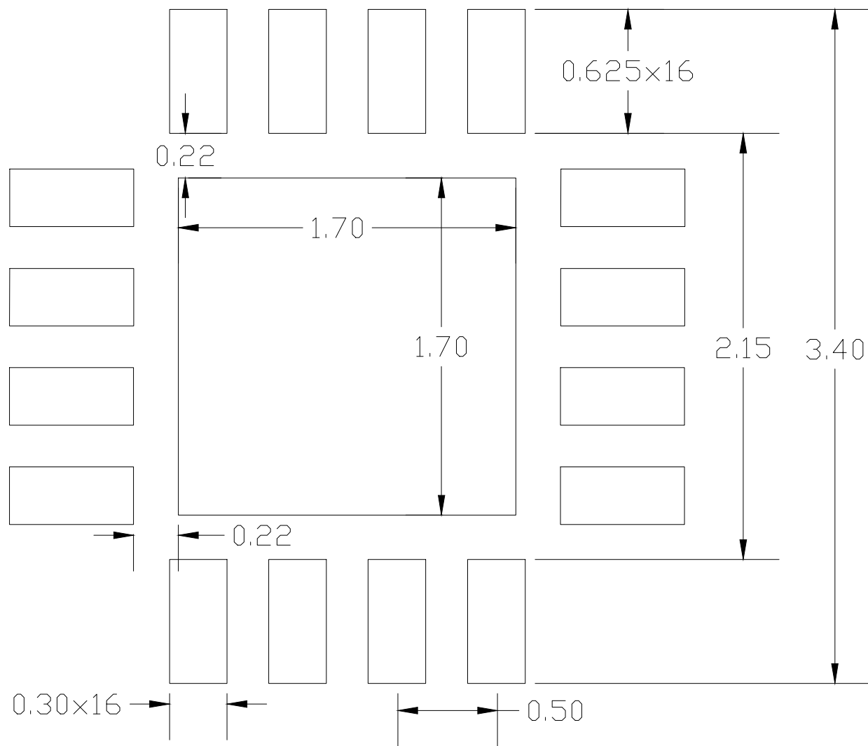
TYPICAL RECOMMENDED LAND PATTERN
