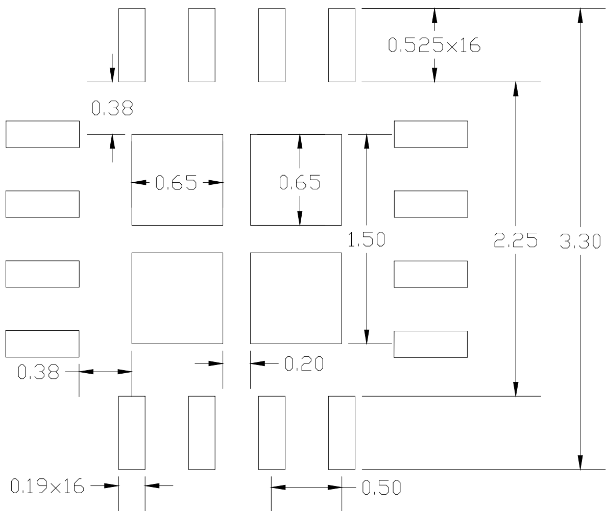
TYPICAL RECOMMENDED STENCIL
